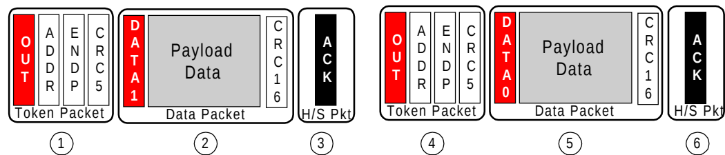
Figure 1-3. USB Packet
