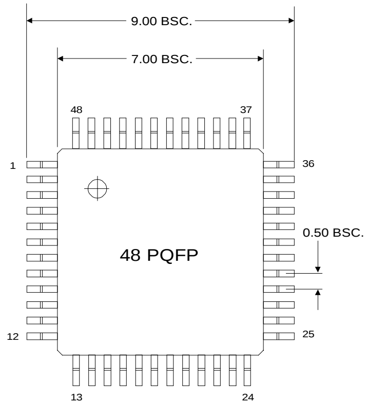
Figure 14-8. 48-Pin PQFP Package (Top View)
