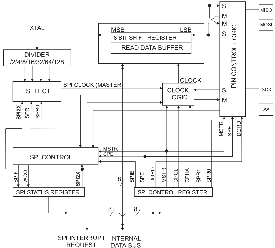
Figure 75. SPI 方框图 (1)
