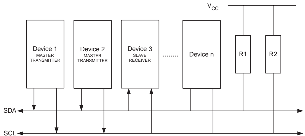
Figure 105. 仲裁示例
