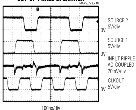
OUT-OF-PHASE OPERATION
