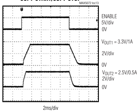
SOFT-START/SOFT-STOP
