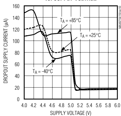
DROPOUT SUPPLY CURRENT vs. SUPPLY VOLTAGE
