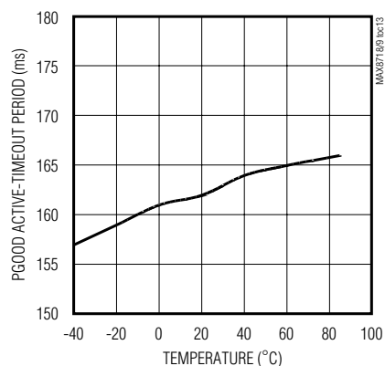
PGOOD ACTIVE-TIMEOUT PERIOD vs. TEMPERATURE
