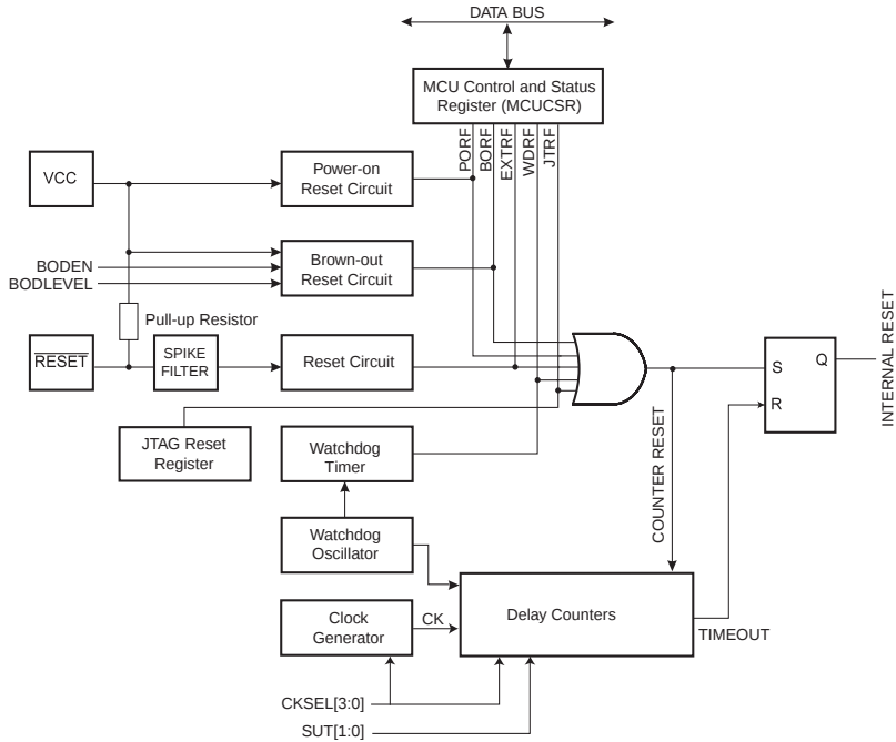
Figure 15. 复位逻辑
