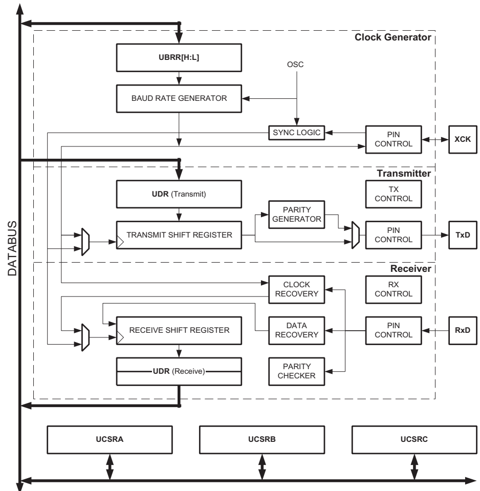
Figure 69. USART 方框图 (1)
