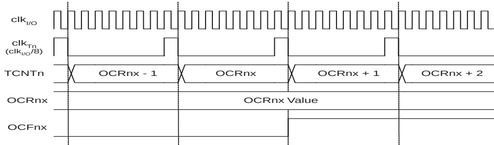
Figure 63. T/C 时序图，OCF2A 置位，预分频器为 f_{\text{clk}_{I/O}}/8
