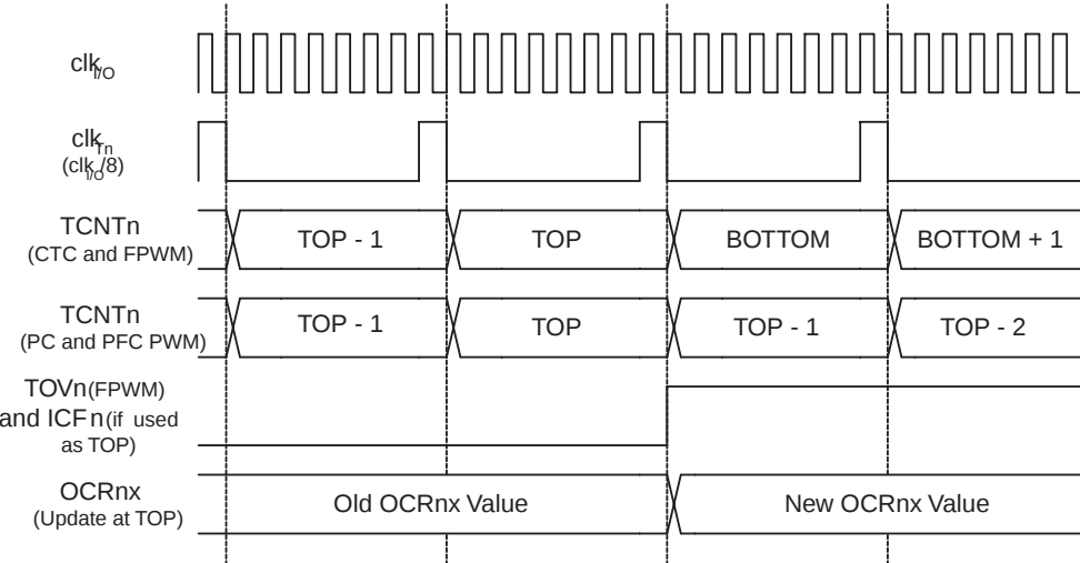
Figure 53. T/C 时序图，预分频器为 f_{clk\_I/O}/8
