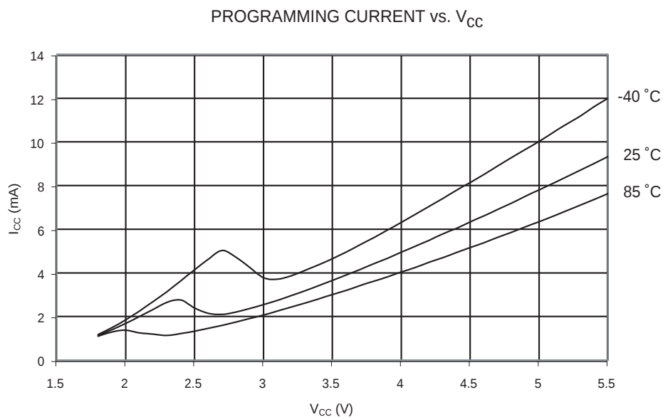
Figure 177. Programming Current vs. V_{CC}
