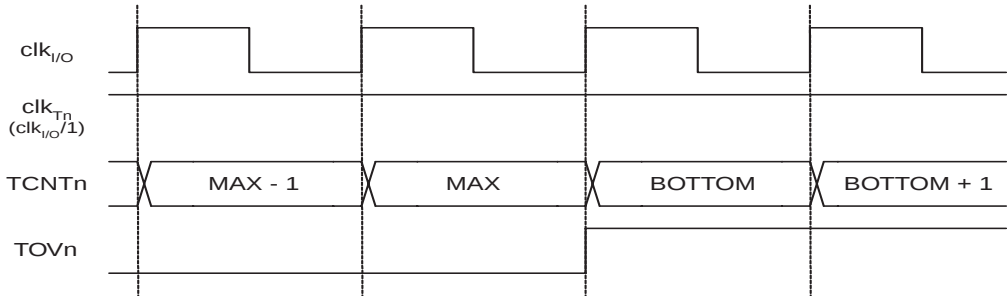
Figure 61. T/C 时序图，无预分频器
