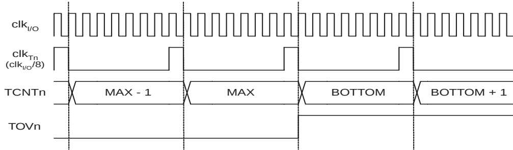
Figure 62. T/C 时序图，预分频器为 f_{\text{clk}_{I/O}}/8
