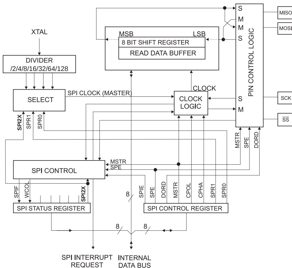
Figure 66. SPI 方框图 (1)
