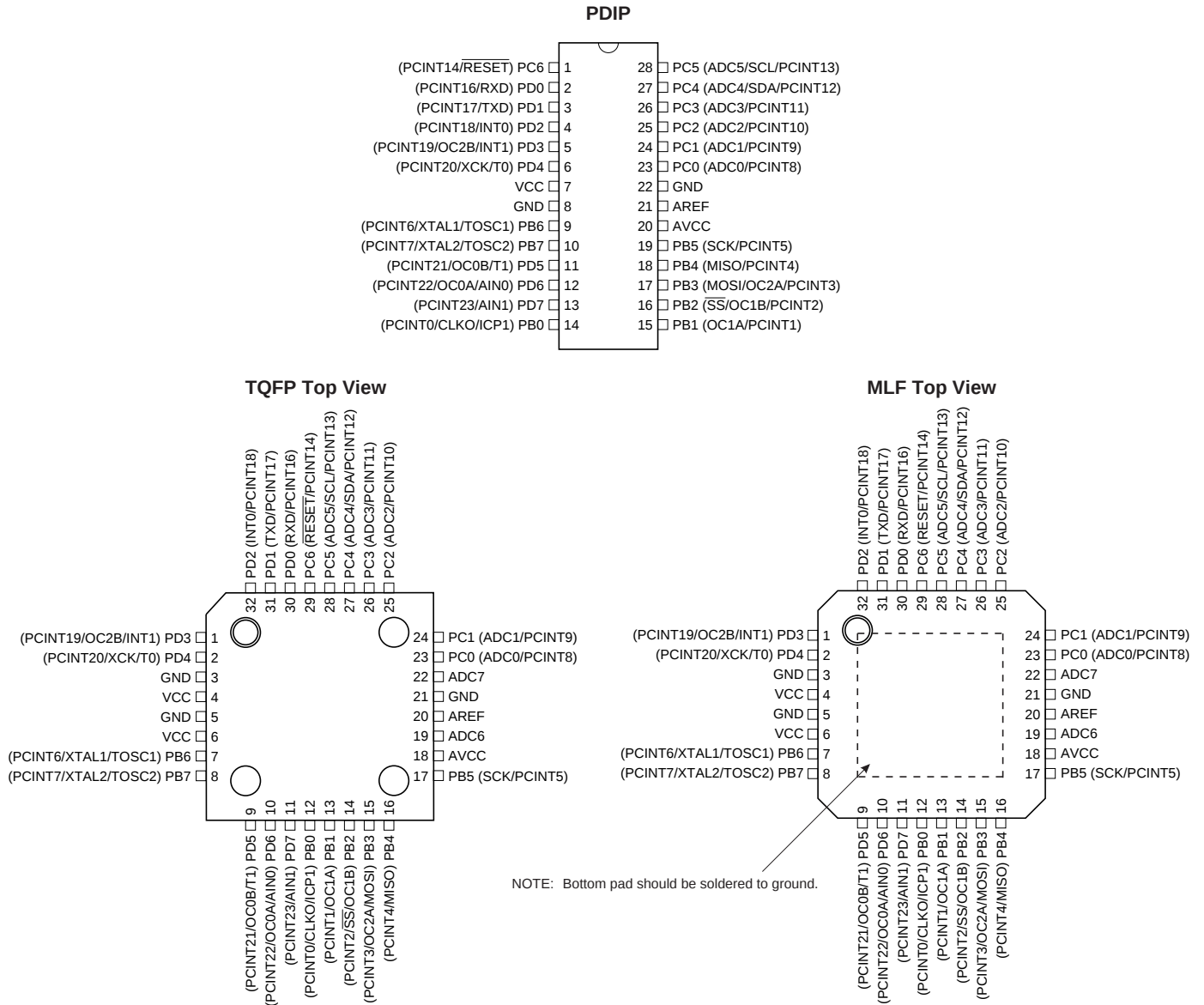
Figure 1. ATmega48/88/168 引脚排列
