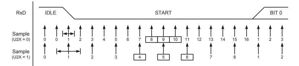
Figure 74. 起始位采样
