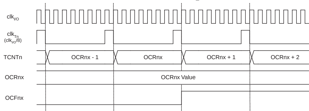
Figure 37. T/C 时序图，OCF0x 置位，预分频器为 f_{clk\_I/O}/8
