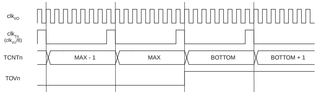
Figure 36. T/C 时序图，预分频器为 f_{\text{clk\_I/O}}/8
