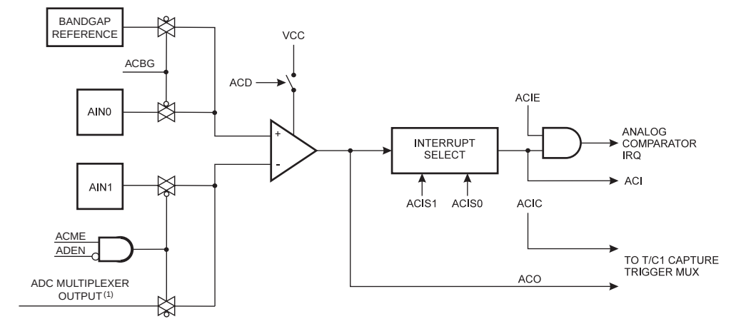
Figure 100. 模拟比较器框图 (2)
