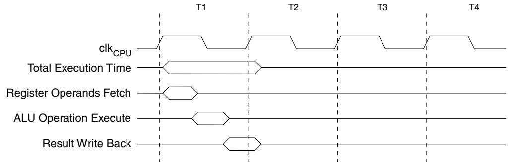
Figure 6. Single Cycle ALU Operation
