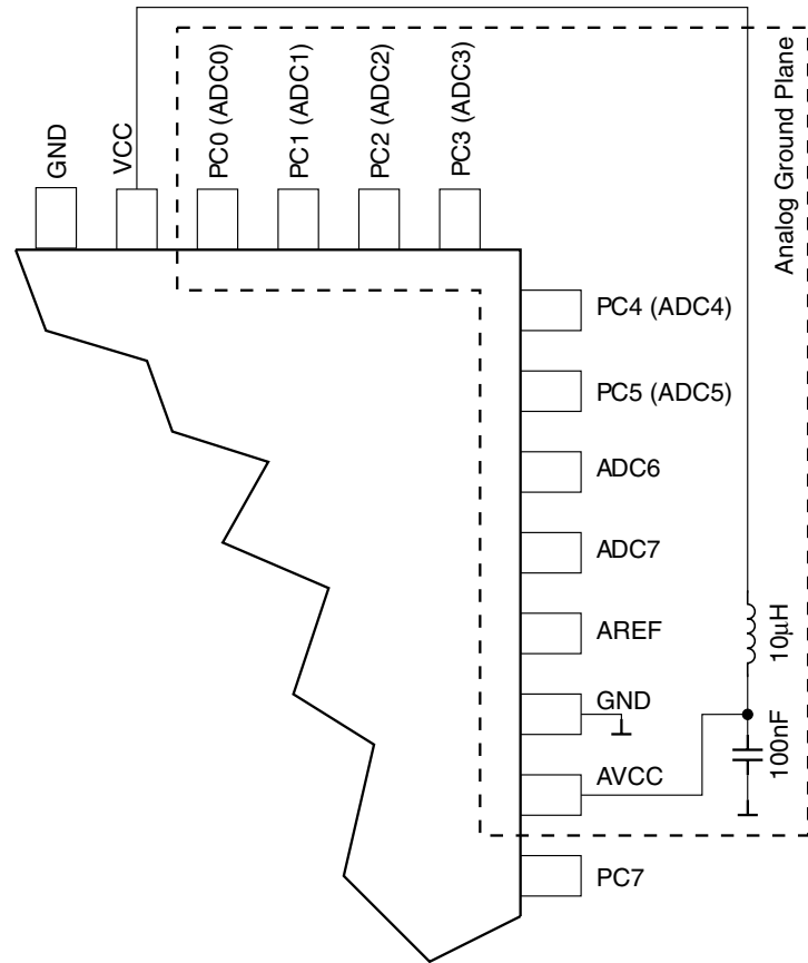
Figure 96. ADC Power Connections
