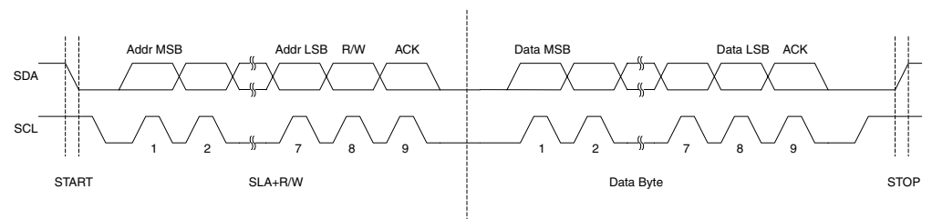
Figure 73. Typical Data Transmission
