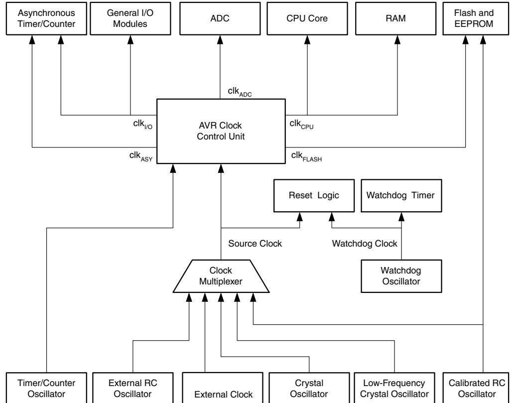
Figure 10. Clock Distribution
