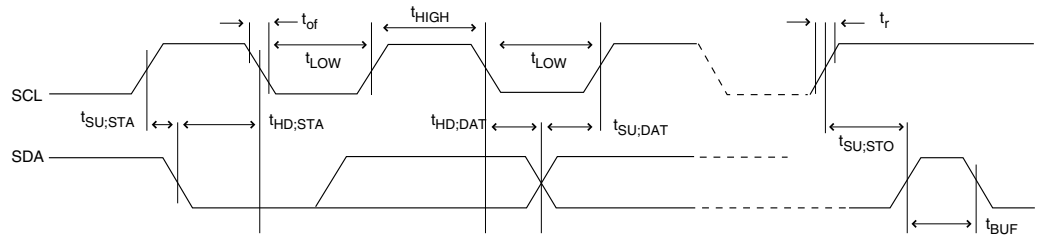
Figure 116. 2-wire Serial Bus Timing
