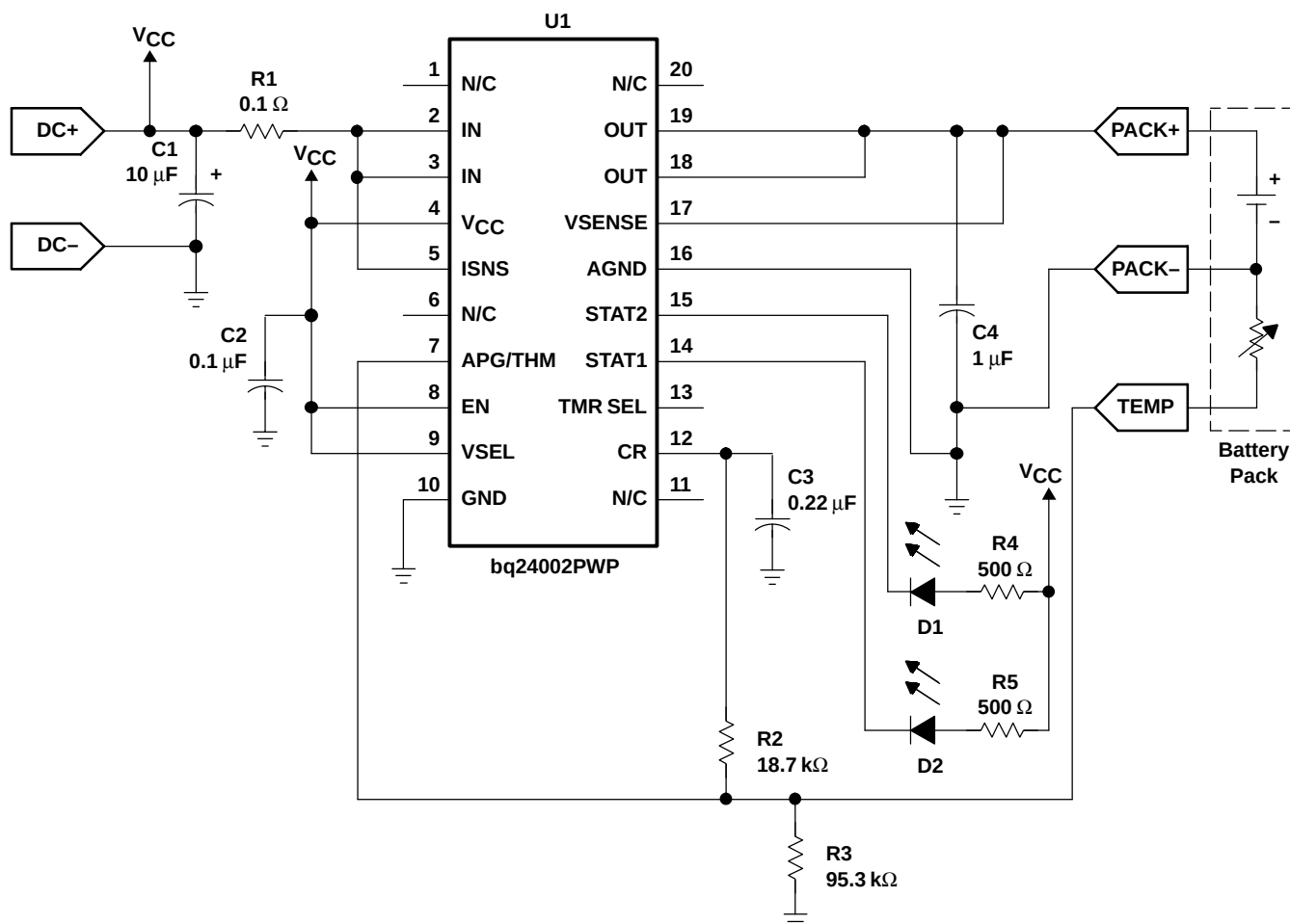
Figure 13. Li-Ion/Li-Pol Charger
