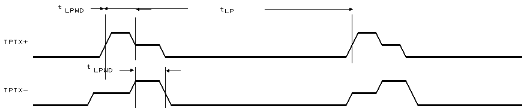
Transmitted Link Integrity Pulse Timing
