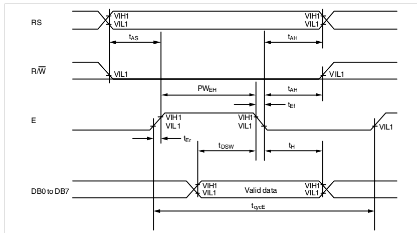
Write Operation
