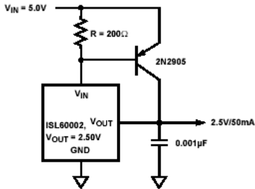
FIGURE 5. PRECISION 2.5V 50mA REFERENCE
