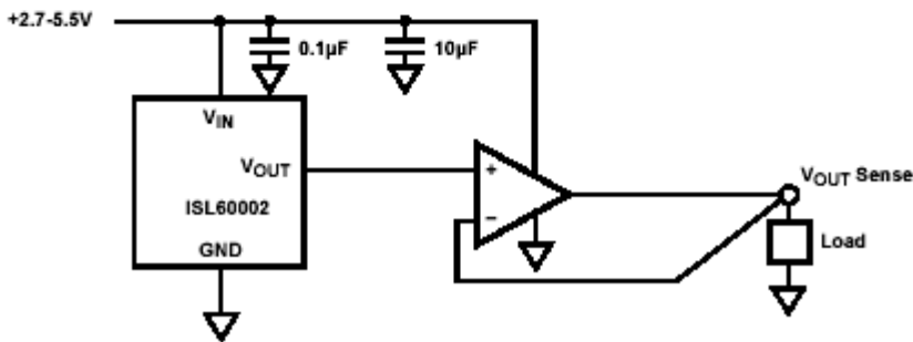
FIGURE 7. KELVIN SENSED LOAD
