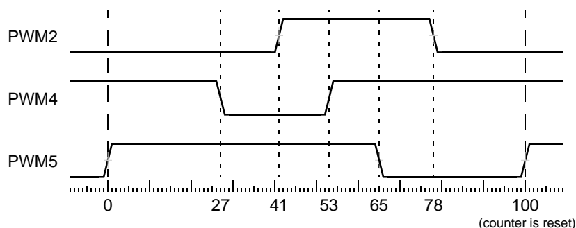
Figure 40: Sample PWM waveforms
