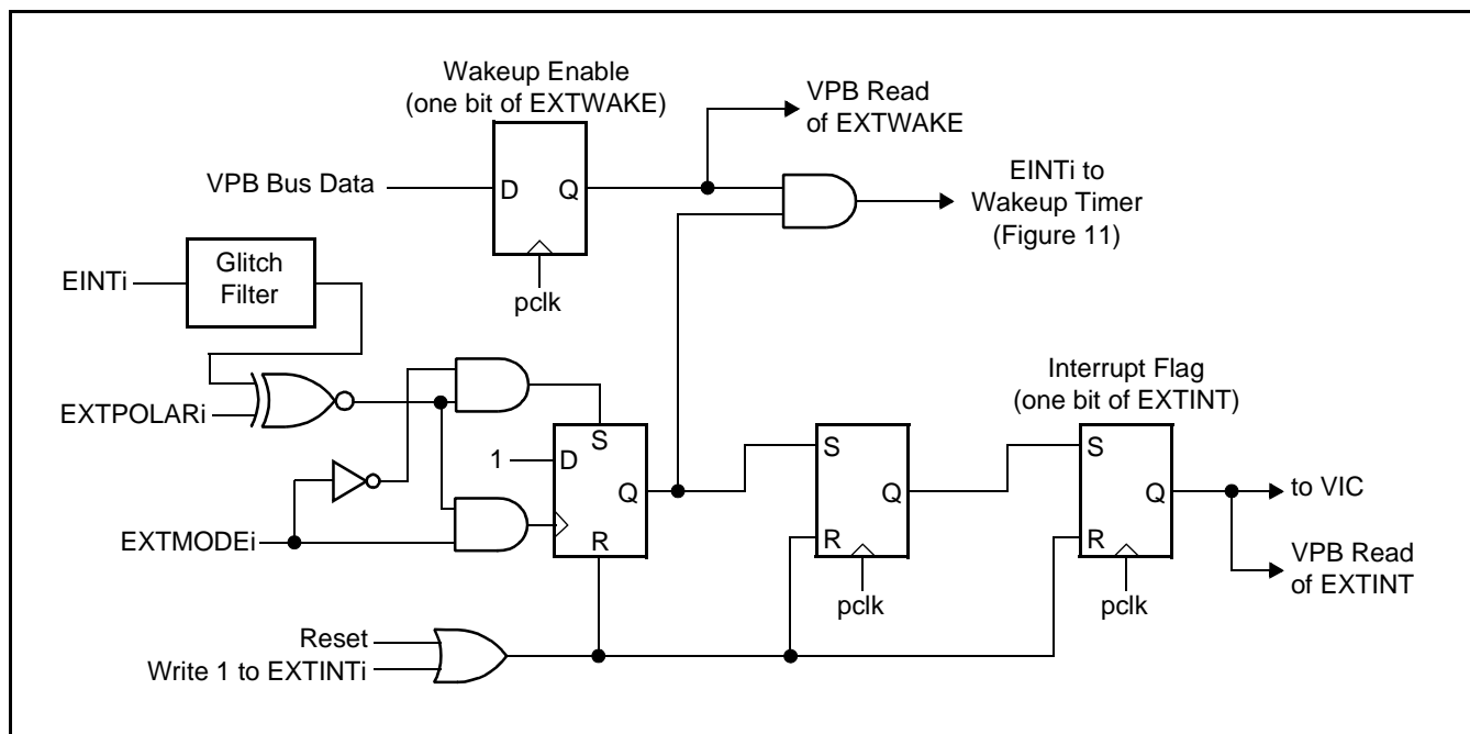
Figure 9: External Interrupt Logic
