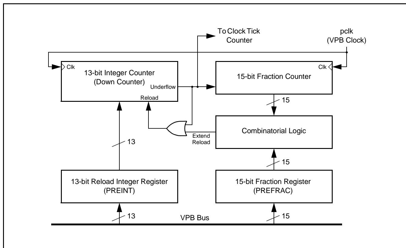
Figure 42: RTC Prescaler block diagram
