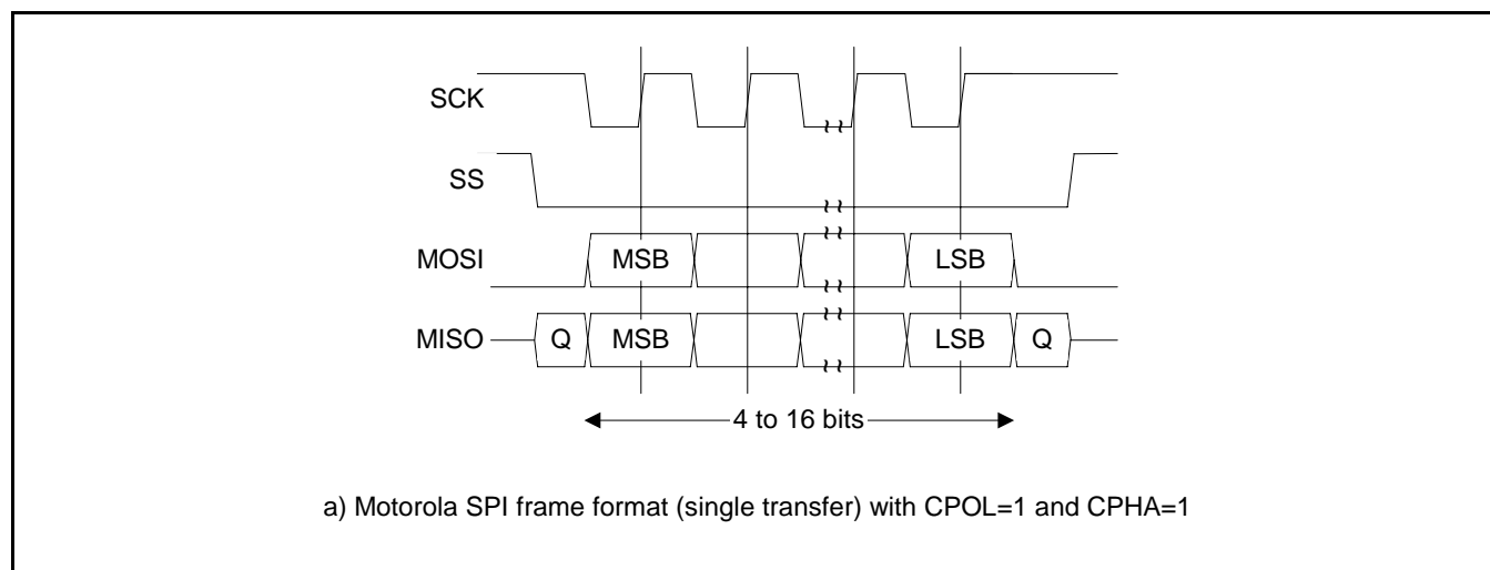
Figure 32: SPI frame format with CPOL=1 and CPHA=1
