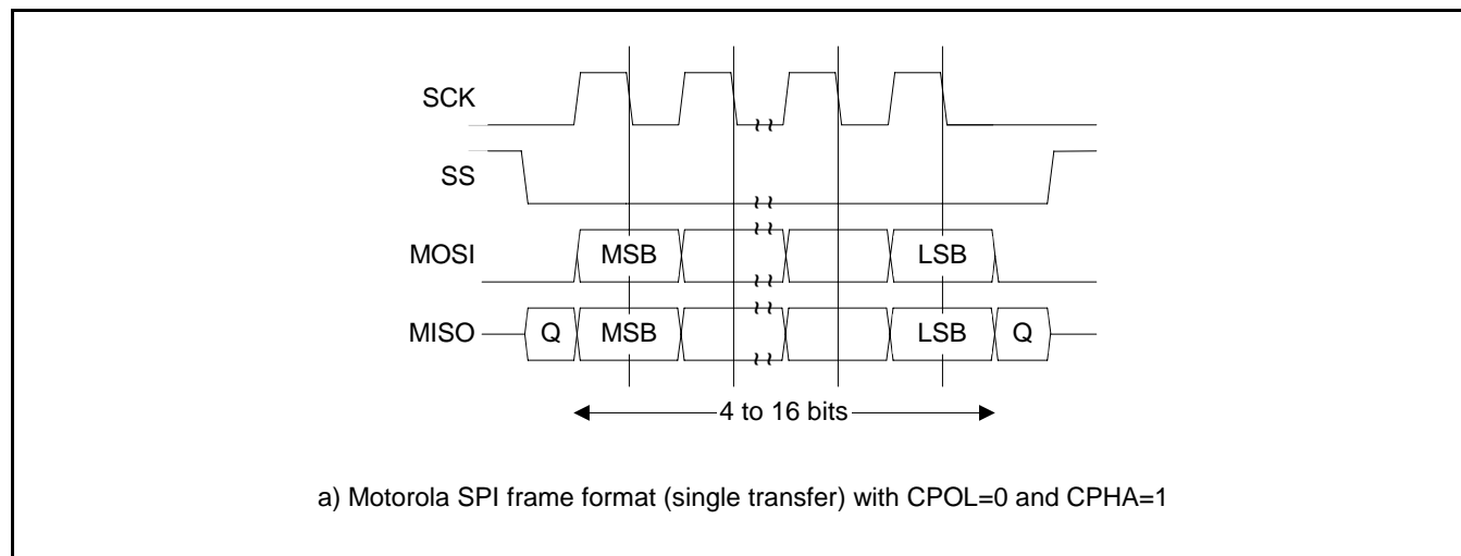
Figure 30: SPI frame format with CPOL=0 and CPHA=1
