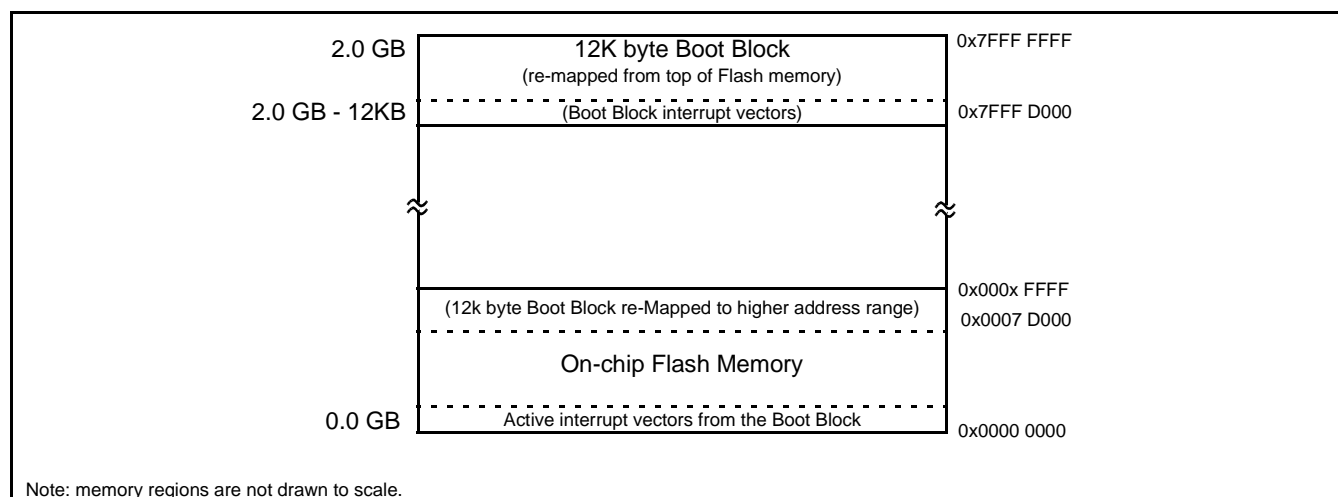
Figure 163: Map of lower memory after reset
