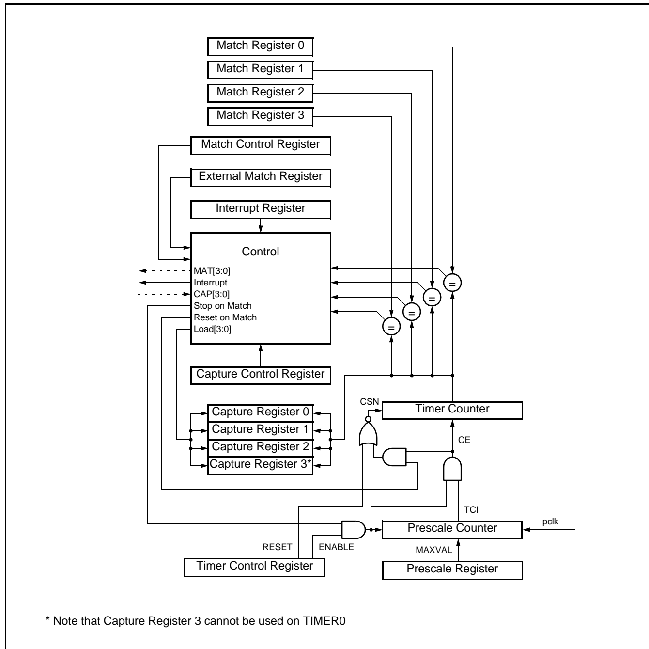
Figure 38: Timer block diagram
