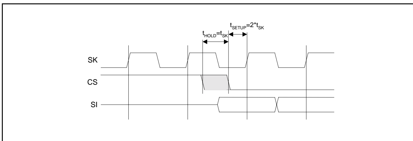
Figure 35: Microwire frame format (continuous transfers)
