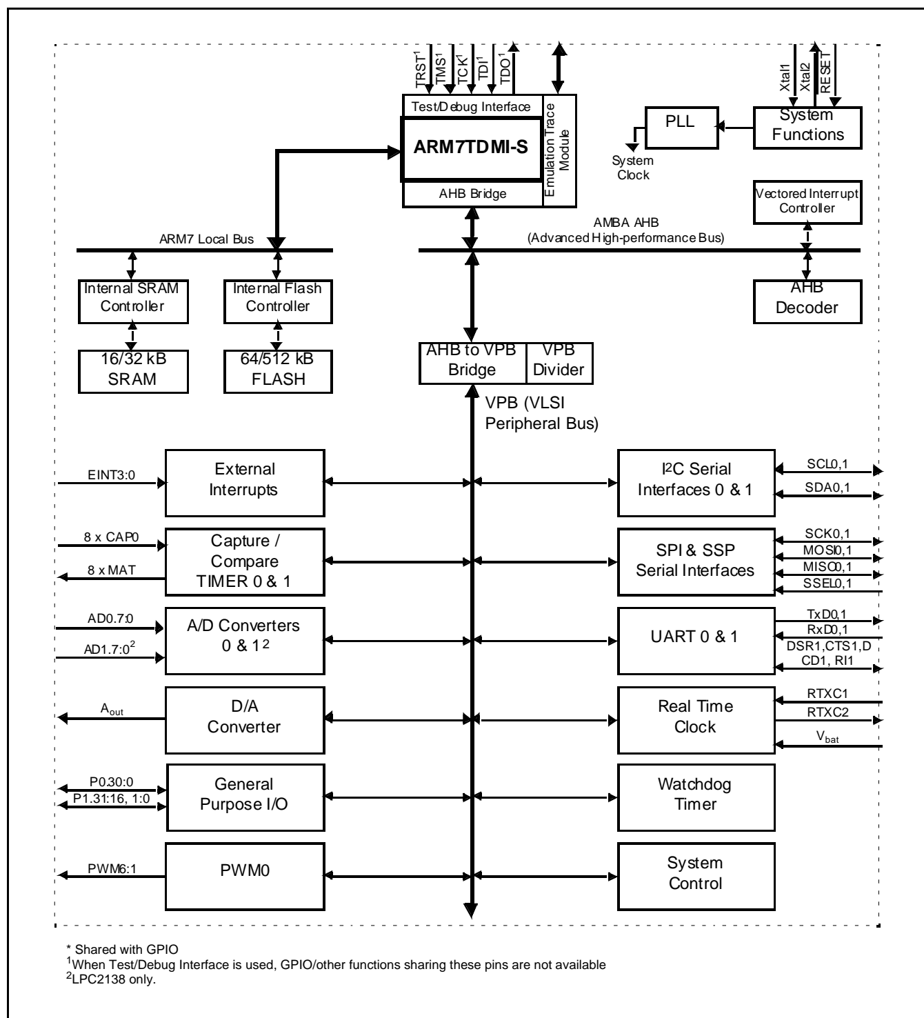
Figure 1: LPC2132/2138 Block Diagram
