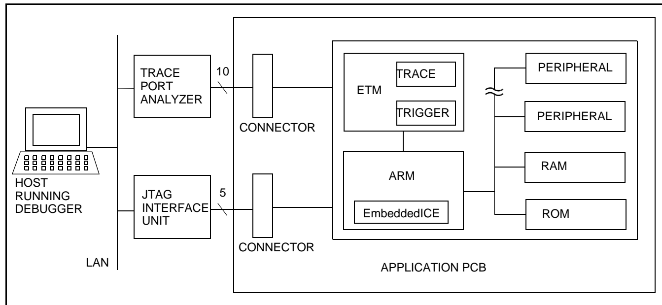
Figure 2: ETM Debug Environment Block Diagram
