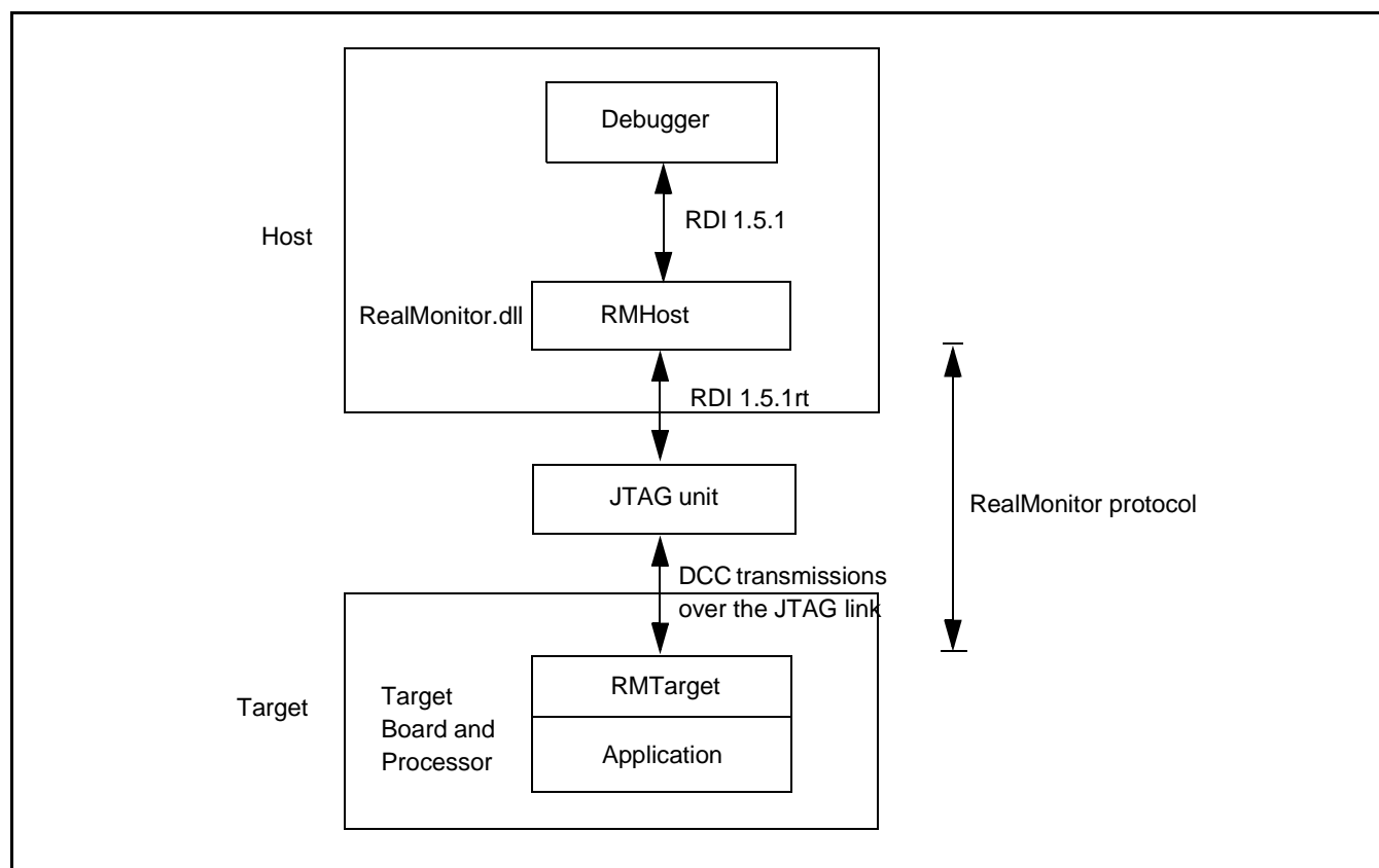
Figure 3: RealMonitor components
