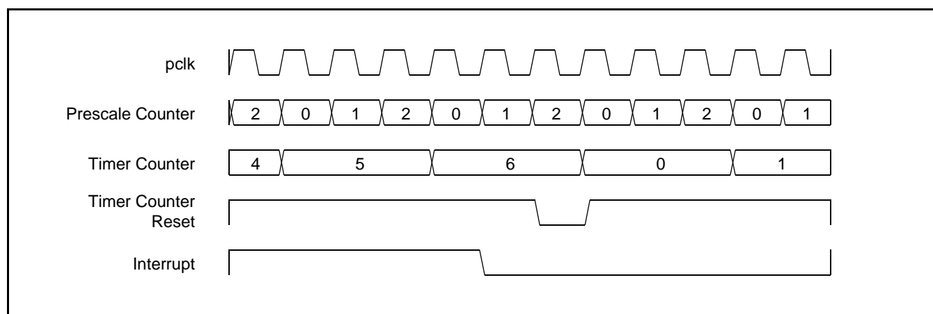
Figure 36: A timer cycle in which PR=2, MRx=6, and both interrupt and reset on match are enabled.
