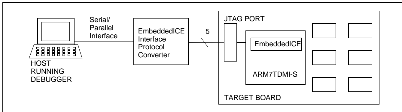
Figure 1: EmbeddedICE Debug Environment Block Diagram
