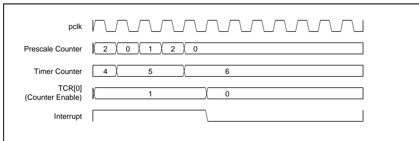
Figure 37: A timer cycle in which PR=2, MRx=6, and both interrupt and stop on match are enabled.
