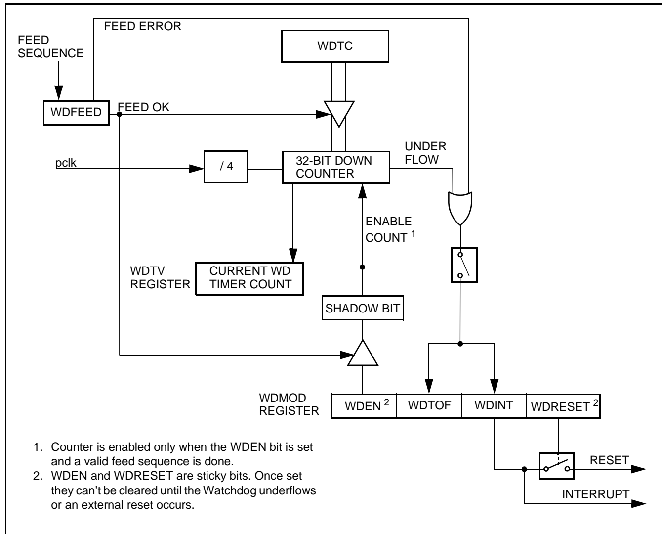
Figure 43: Watchdog Block Diagram
