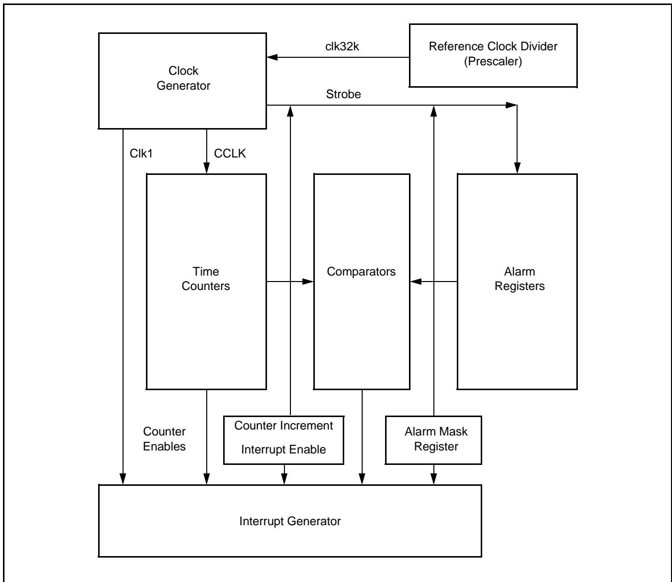
Figure 41: RTC block diagram
