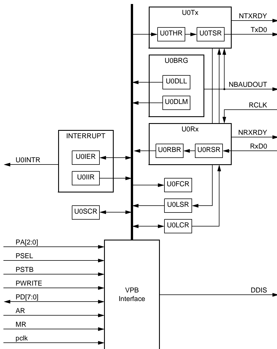
Figure 15: LPC2210 UART0 Block Diagram
