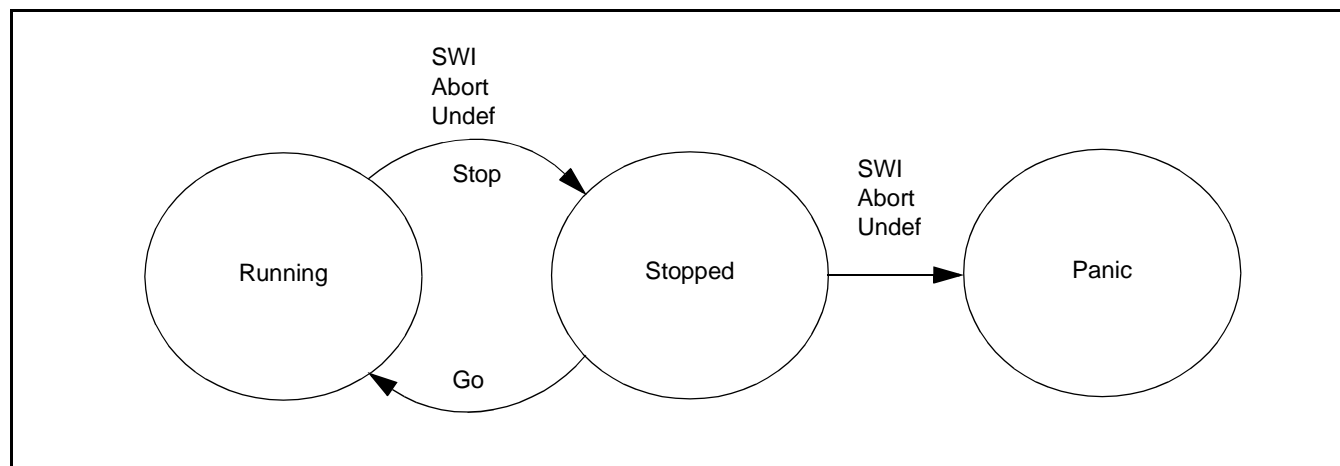
Figure 4: RealMonitor as a state machine
