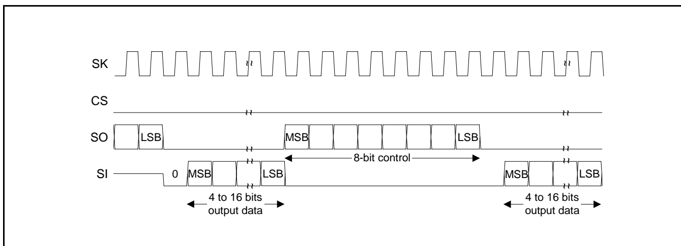
Figure 34: Microwire frame format (continuous transfers)
