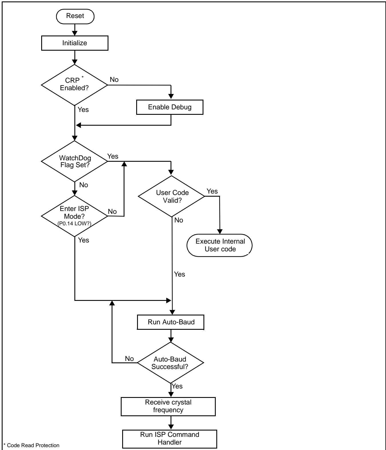
Figure 164: Boot Process flowchart
