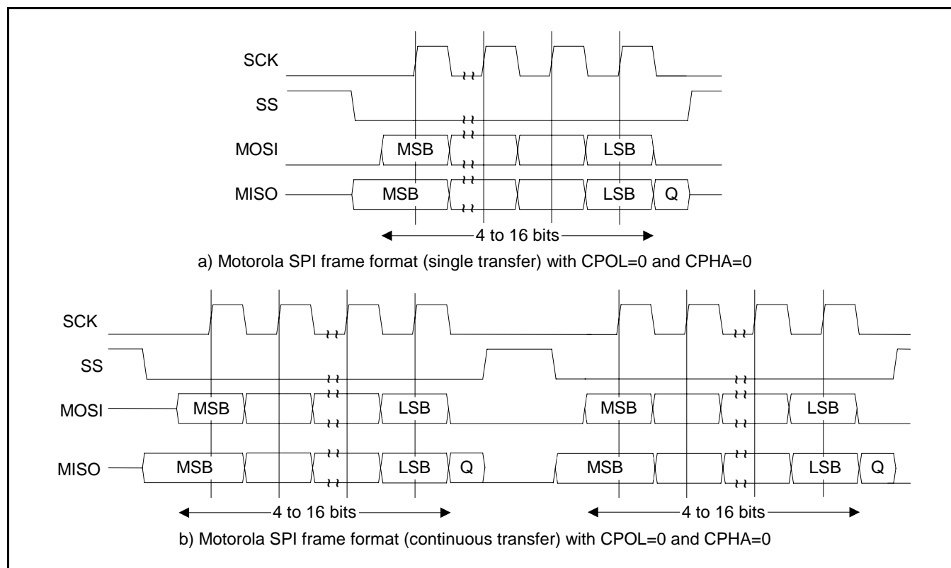
Figure 29: SPI frame format with CPOL=0 and CPHA=0 (a) single and b) continuous transfer)
