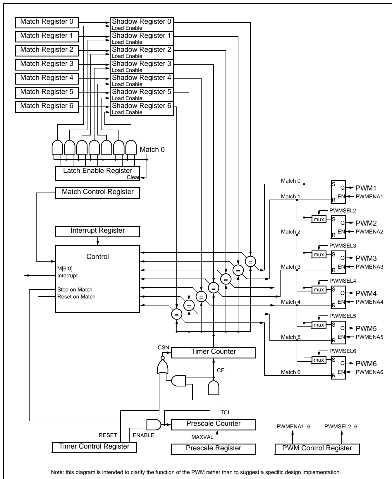
Figure 39: PWM block diagram
