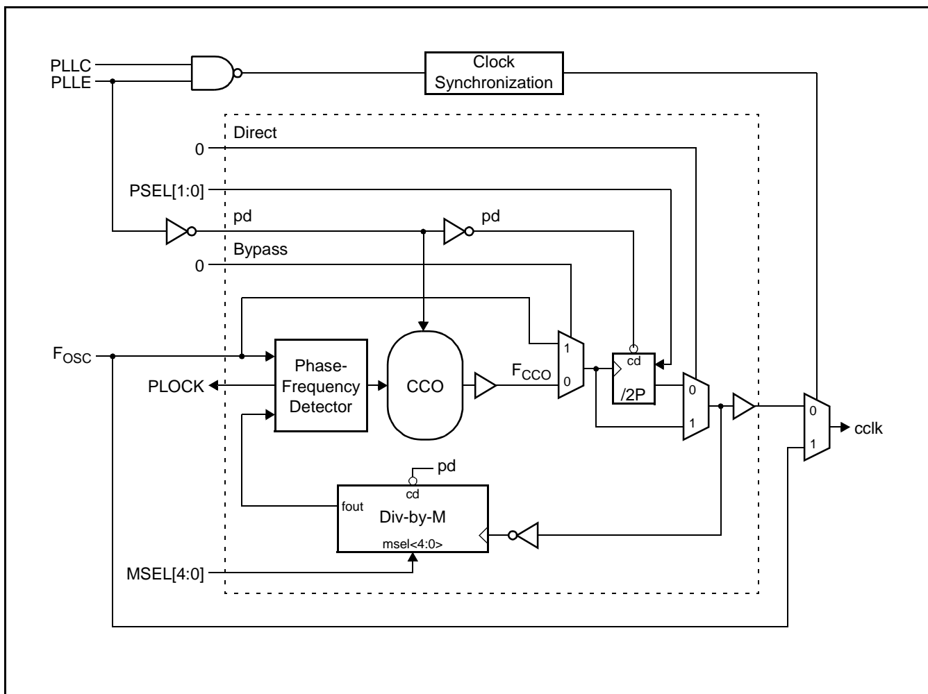
Figure 10: PLL Block Diagram
