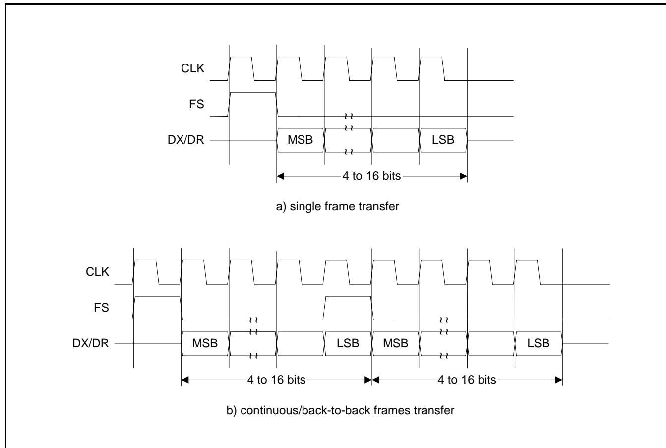
Figure 28: Texas Instruments synchronous serial frame format: a) single and b) continuous/back-to-back two frames transfer
