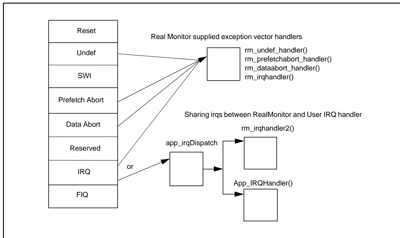
Figure 5: Exception Handlers
