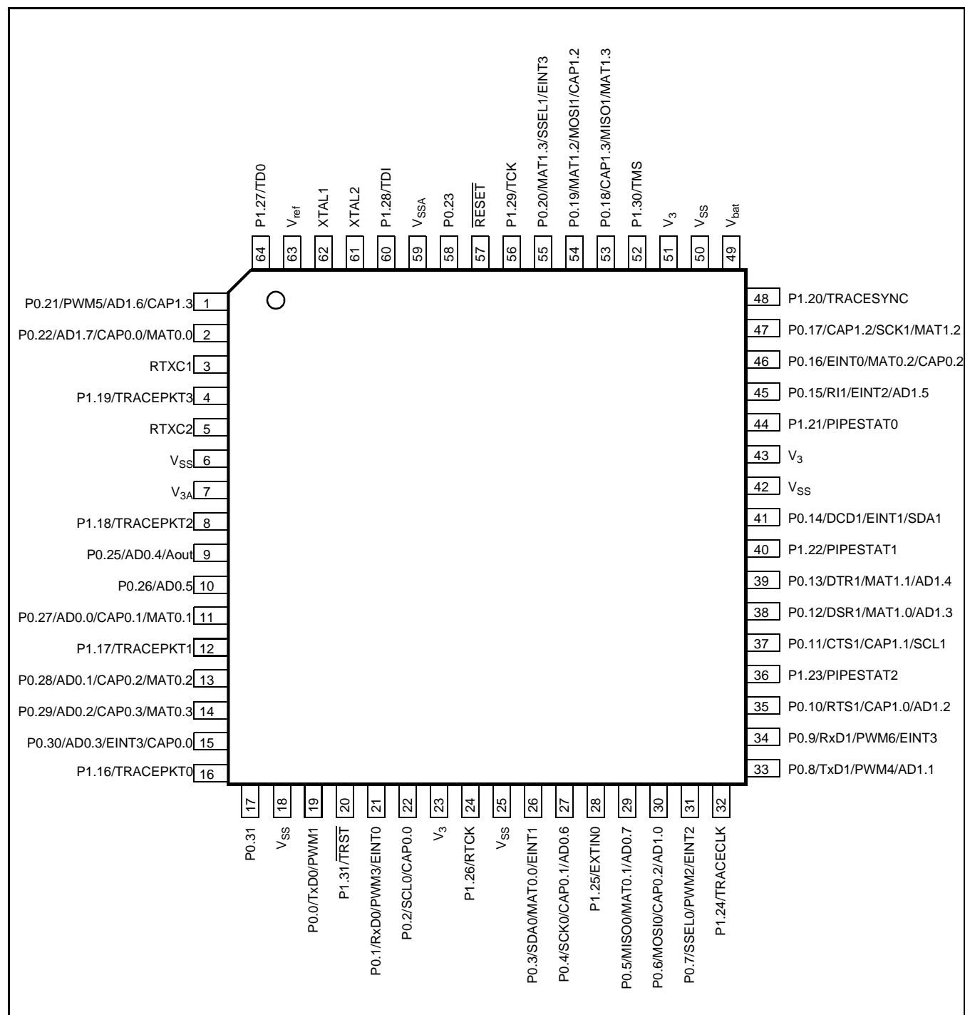
Figure 14: LPC2132/2138 64-pin package
