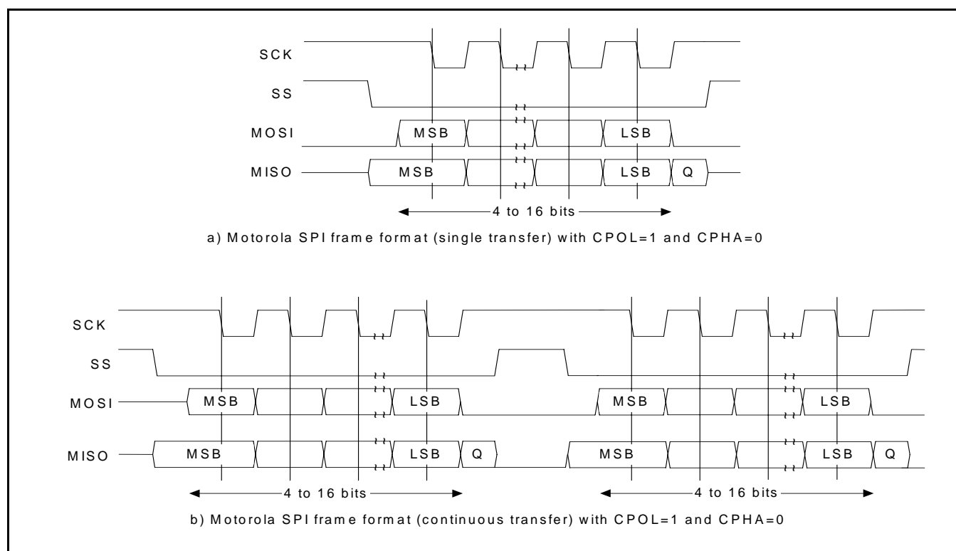
Figure 31: SPI frame format with CPOL=1 and CPHA=0 (a) single and b) continuous transfer)
