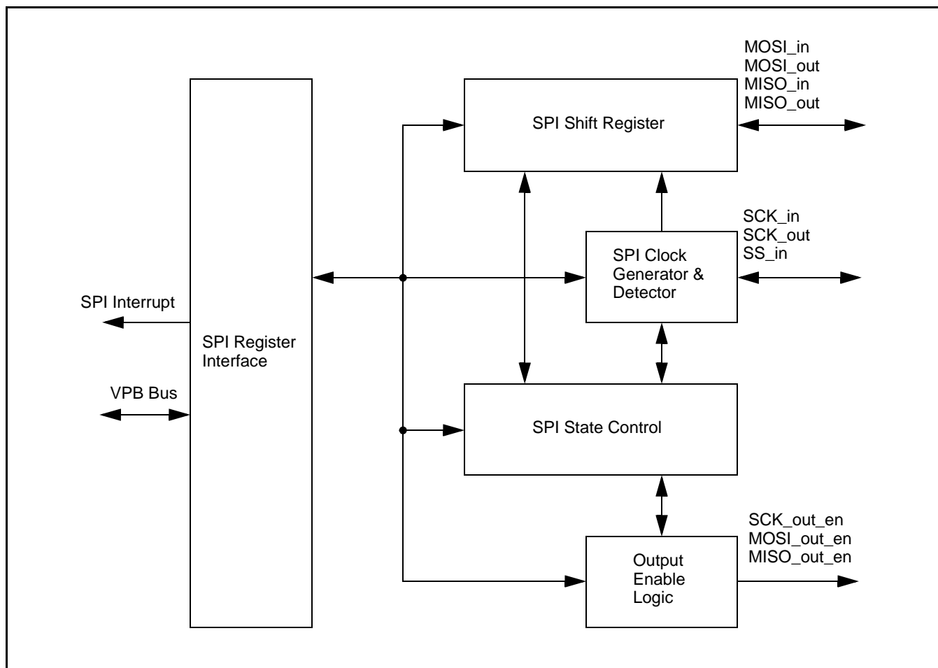
Figure 27: SPI Block Diagram
