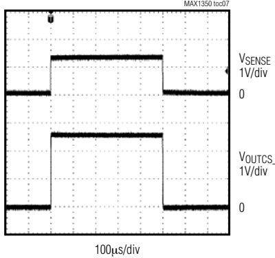
SENSE-AMPLIFIER TRANSIENT RESPONSE
