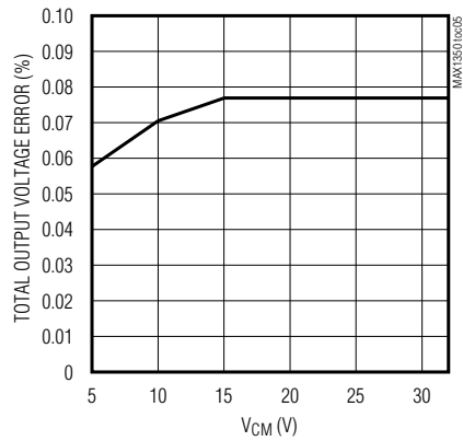
SENSE-AMPLIFIER TOTAL OUTPUT VOLTAGE ERROR vs. COMMON-MODE VOLTAGE
