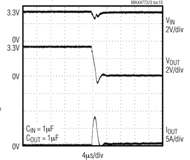
CURRENT-LIMIT RESPONSE (OUT SHORTED TO GND)
