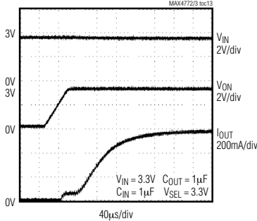
CURRENT-LIMIT RESPONSE
