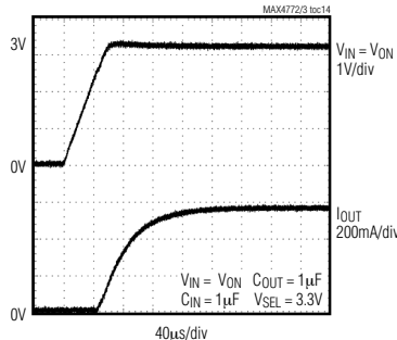
CURRENT-LIMIT RESPONSE
