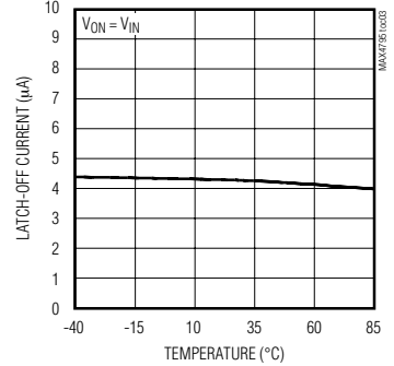
LATCH-OFF LEAKAGE CURRENT vs. TEMPERATURE
