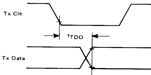
FIGURE 3 — TRANSMIT DATA OUTPUT DELAY
