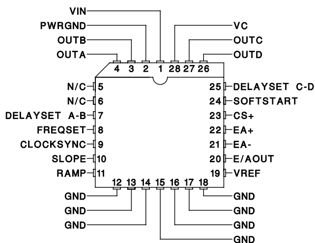
PLCC-28 or CLCC-28 (Top View) QP or L Package
